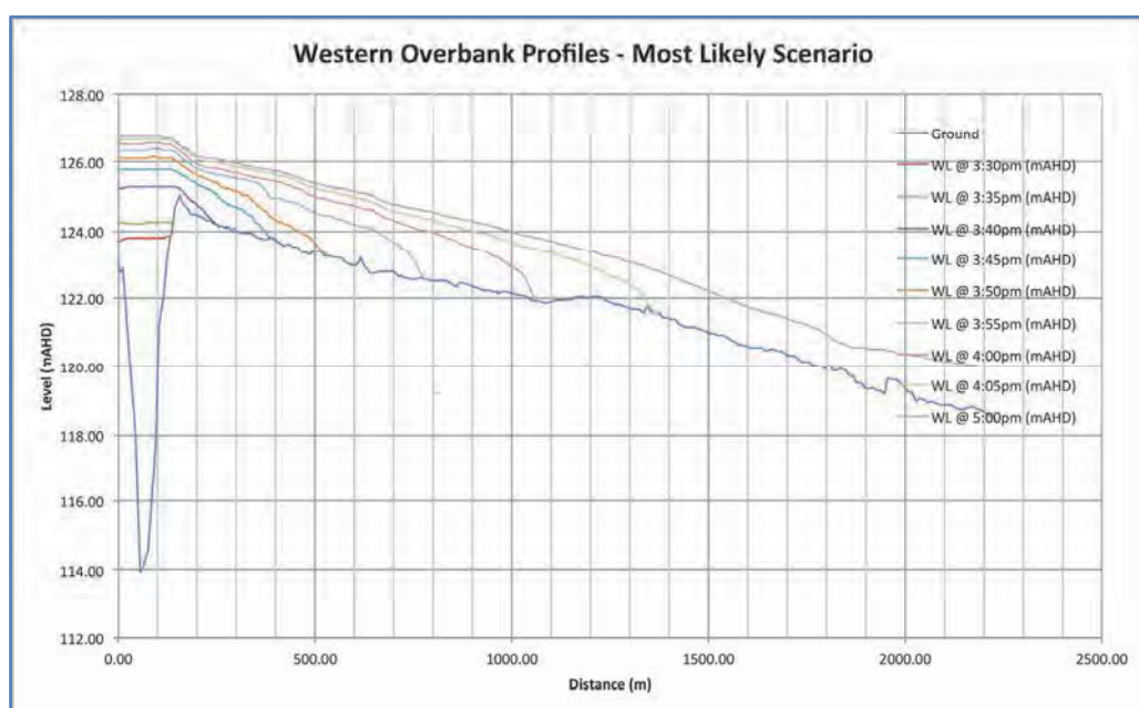
Figure 5.18: Western overbank flow profiles
