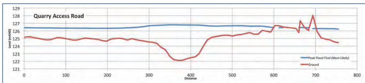
Figure 5.17: Cross-section from north to south along Quarry Access Road
