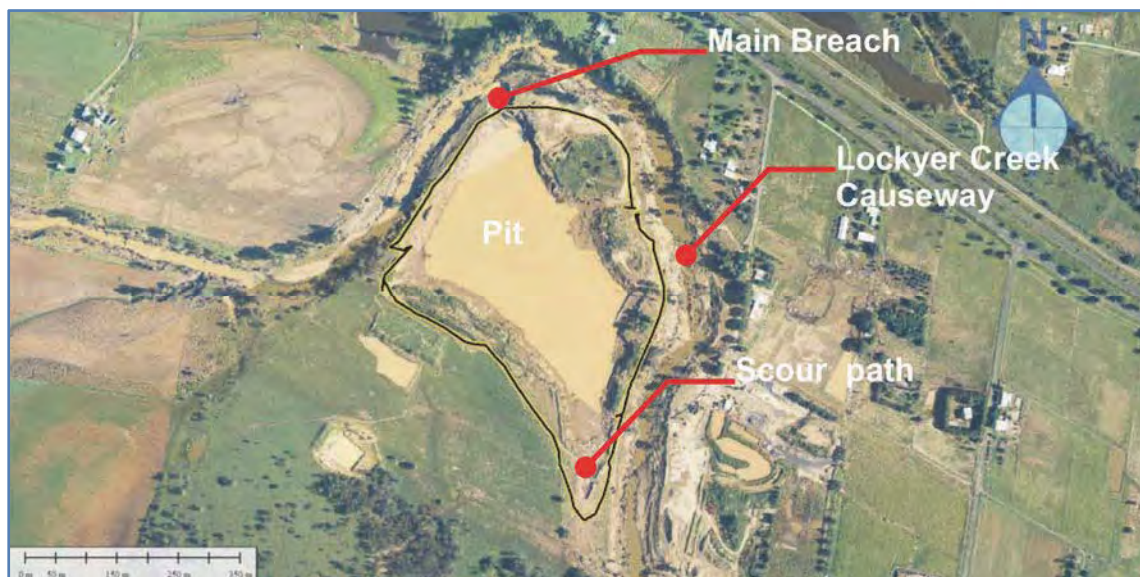
Figure 5.14: Image of Grantham quarry site identifying scour path in south-eastern corner of quarry pit.
