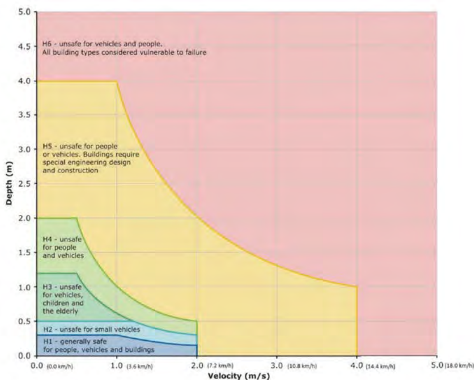
Figure D1: Flood Hazard Vulnerability Curves (AEM, 2014). Source: AEM (2014) Australian Emergency Management Handbook: Managing the Floodplain: best practice in flood risk management in Australia (AEM Handbook 7) available at: https://ema.infoservices.com.au/items/HB7-2ND
