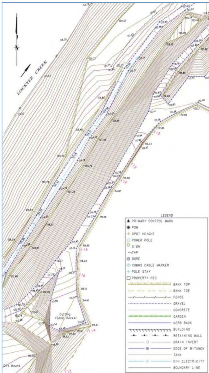
Figure A14: Detail from survey plan of Grantham quarry prepared for Wagners in 2008
