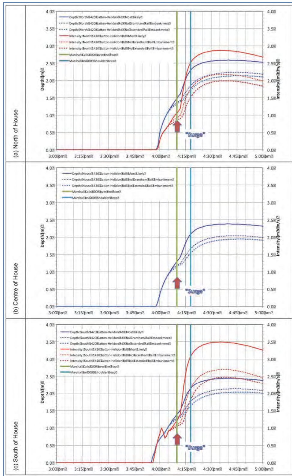
Figure C39: Flow depth intensity at the location of 1420 Gatton-Helidon Road
