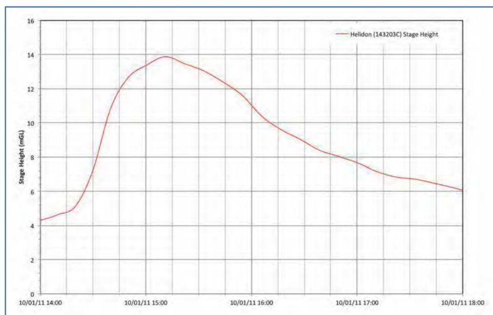
Figure C3: Hydrograph for Helidon stream gauging station on 10 January 2015.
