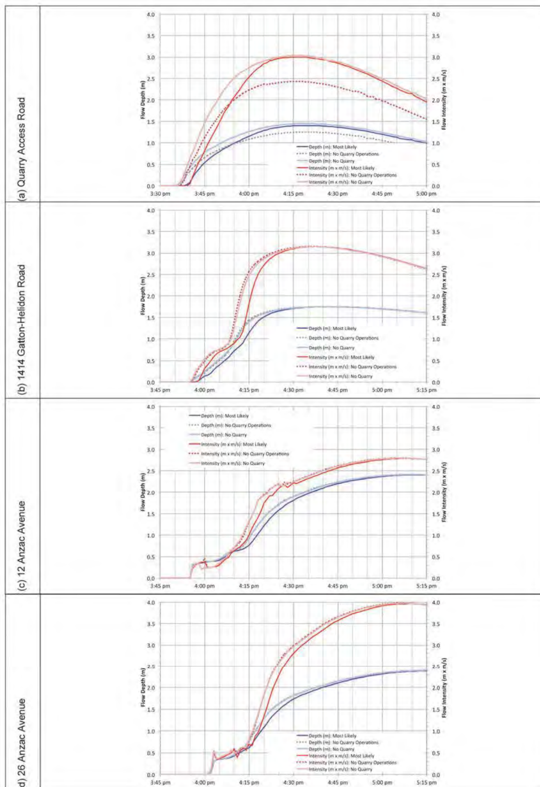
Figure C28: Effect of quarry operations on flow depth and intensity
