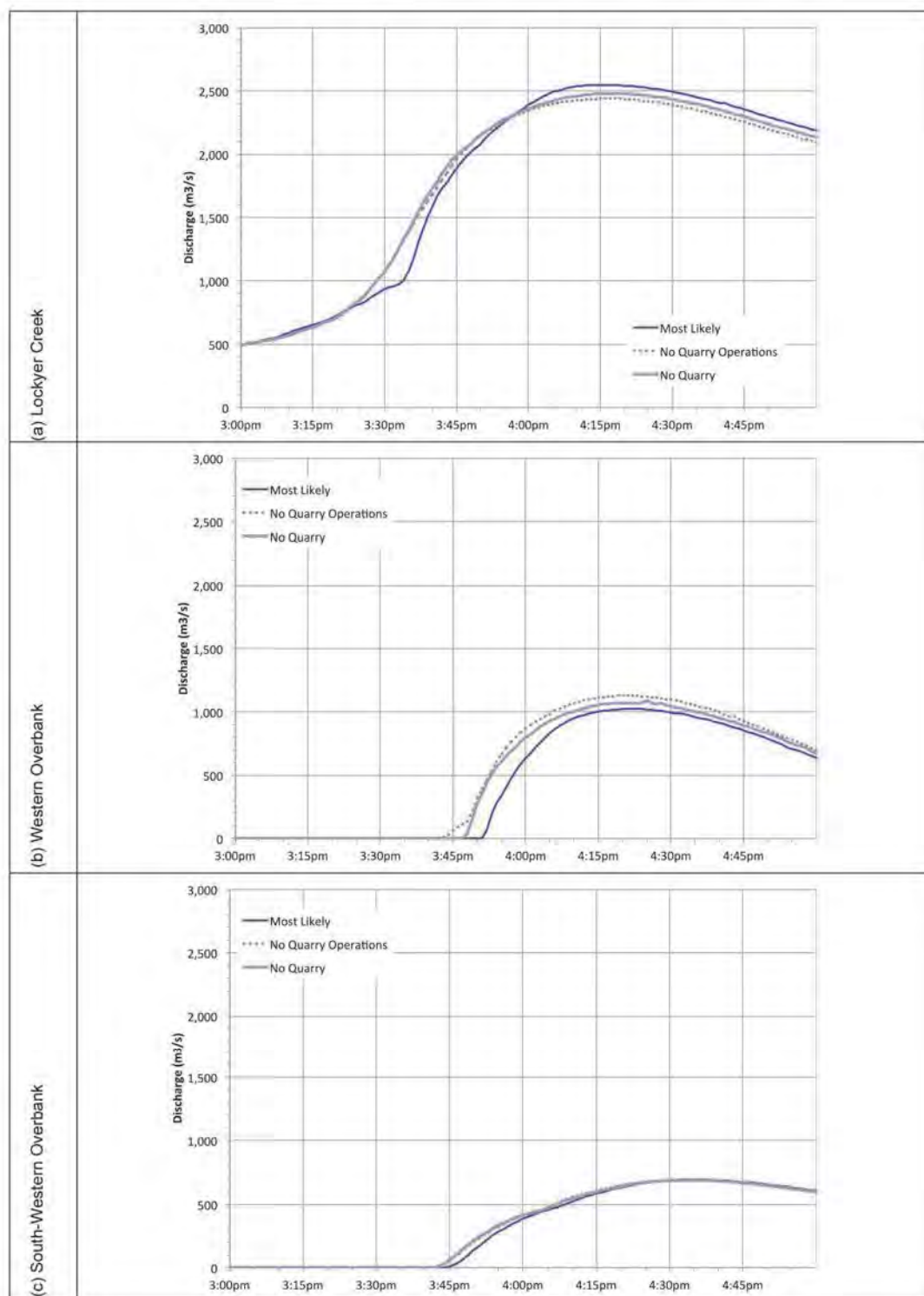
Figure C27: Effect of no quarry operations on downstream flow.
